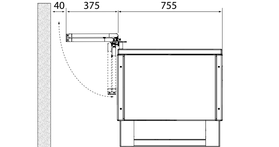
Diagram shows additional space required to stow the neatfold beside the bath
